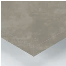
A2-.-16 Front edge with PP edging 1.5 mm thick. 2 x R = 2 mm
